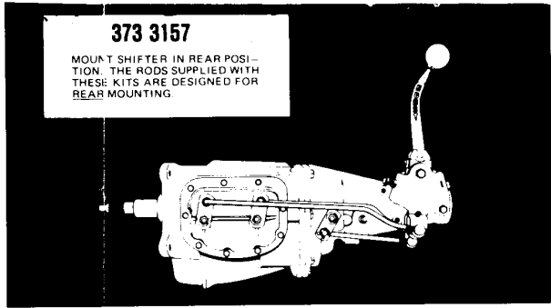
ROD AND REVERSE ARM REQUIRED FOR REAR INSTALLATIONS
