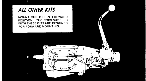
RODS AND REVERSE ARM REQUIRED FOR FORWARD INSTALLATION
